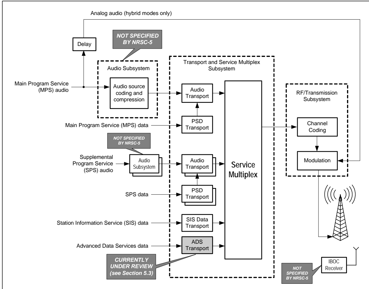
Figure 1: Overview of IBOC digital radio system
