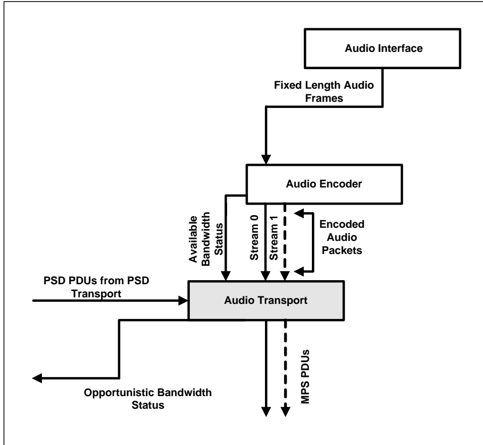
Figure 21: Audio codec protocol interface diagram
