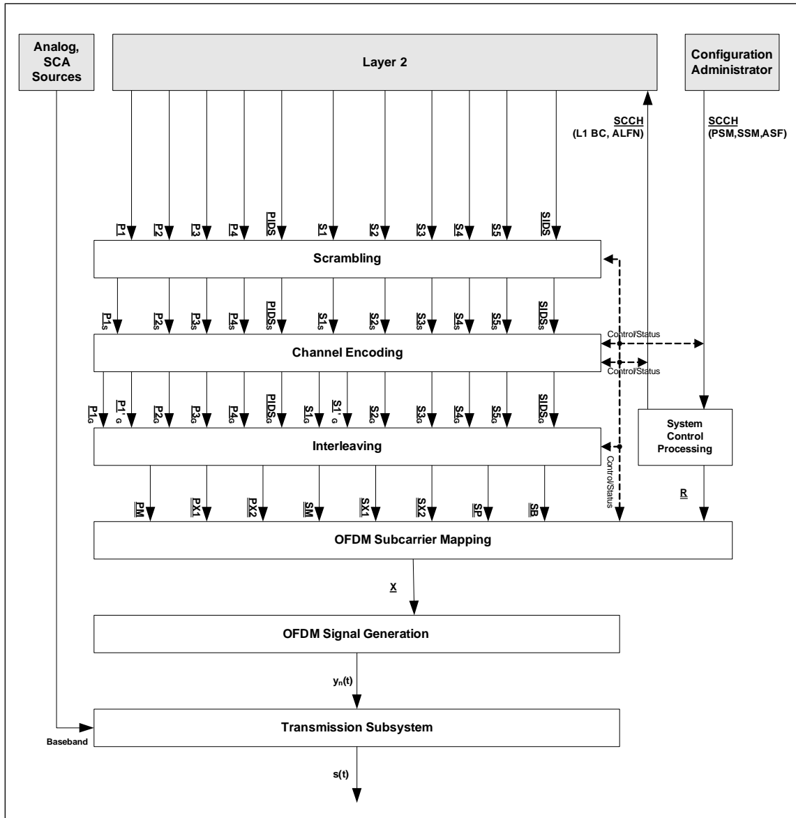
Figure 16: FM band air interface Layer 1 functional block diagram with details of data flow illustrated
