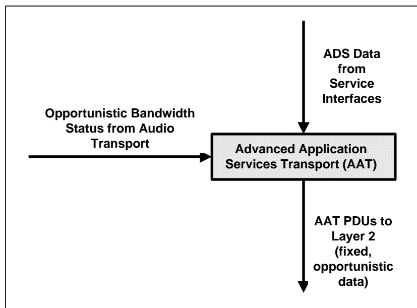
Figure 24. Advanced Data Services Protocol Interface Diagram
