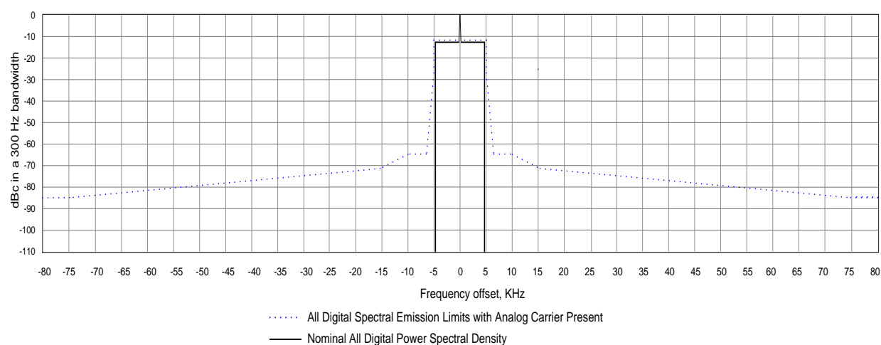
Figure 13. NRSC-5 AM band reduced bandwidth all-digital waveform spectral emissions limits
