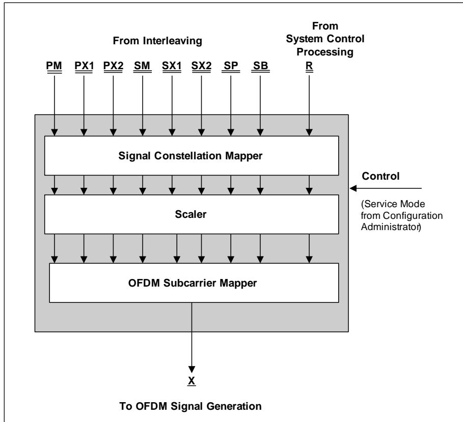
Figure 19: OFDM subcarrier mapping conceptual block diagram
