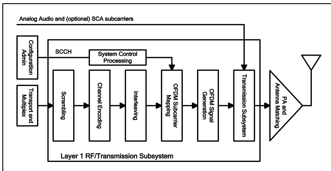
Figure 15: RF/transmission subsystem block diagram
