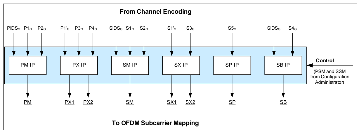
Figure 17: Interleaving conceptual block diagram
