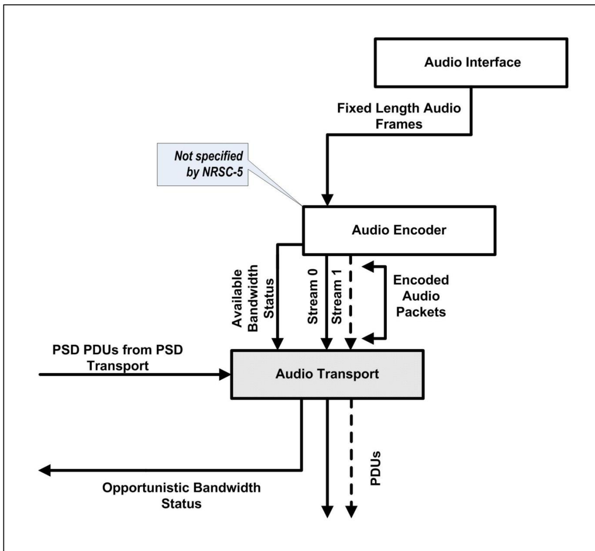
Figure 23: Audio transport interface diagram
