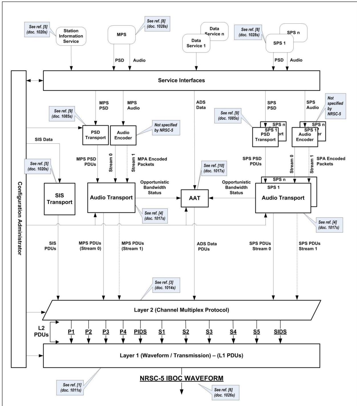
Figure 14: FM band implementation of NRSC-5 IBOC digital radio broadcasting standard
