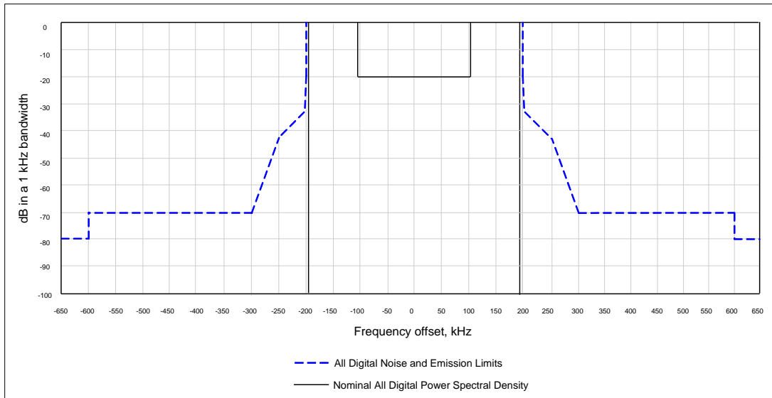
Figure 22. NRSC-5 all-digital waveform noise and emission limits
